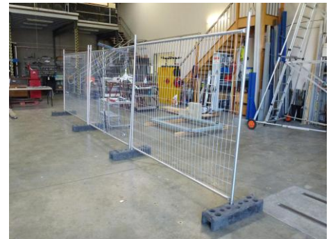
FIG.2 CLIMBING TEST
