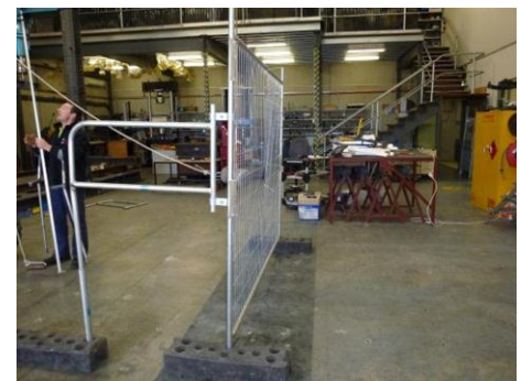
FIG.3 IMPACT TEST
